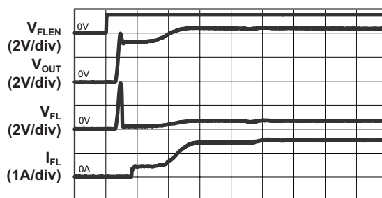
Flash Turn On Characteristic
