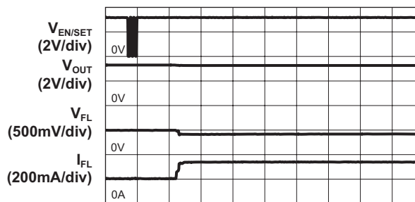
Movie Mode Transition Characteristic
