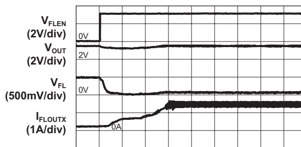
Movie Mode to Flash Turn On Characteristic
