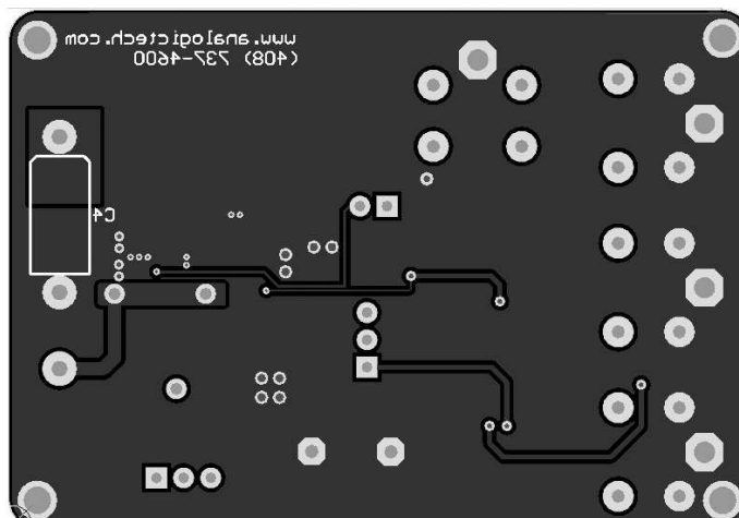
Figure 4: AAT1278 Evaluation Board Bottom Side Layout.
