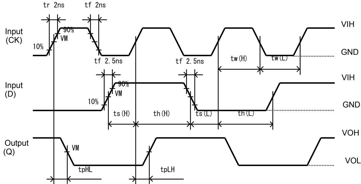
Figure 2 t_{pLH} , t_{pHL}
