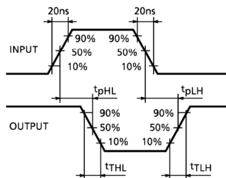
WAVEFORM
