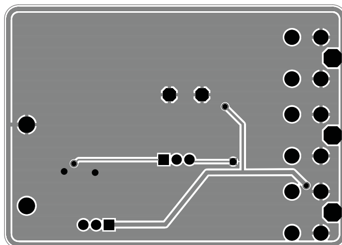
Figure 6: AHK3293 Evaluation Board Bottom Side Layout.
