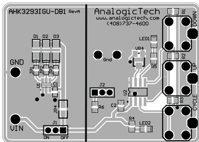
Figure 5: AHK3293 Evaluation Board Top Side Layout.
