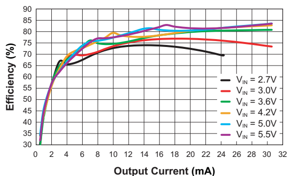
Efficiency vs. Output Current ( R_{SET} = 10K\Omega , L = 10\mu H , 10 LEDs)
