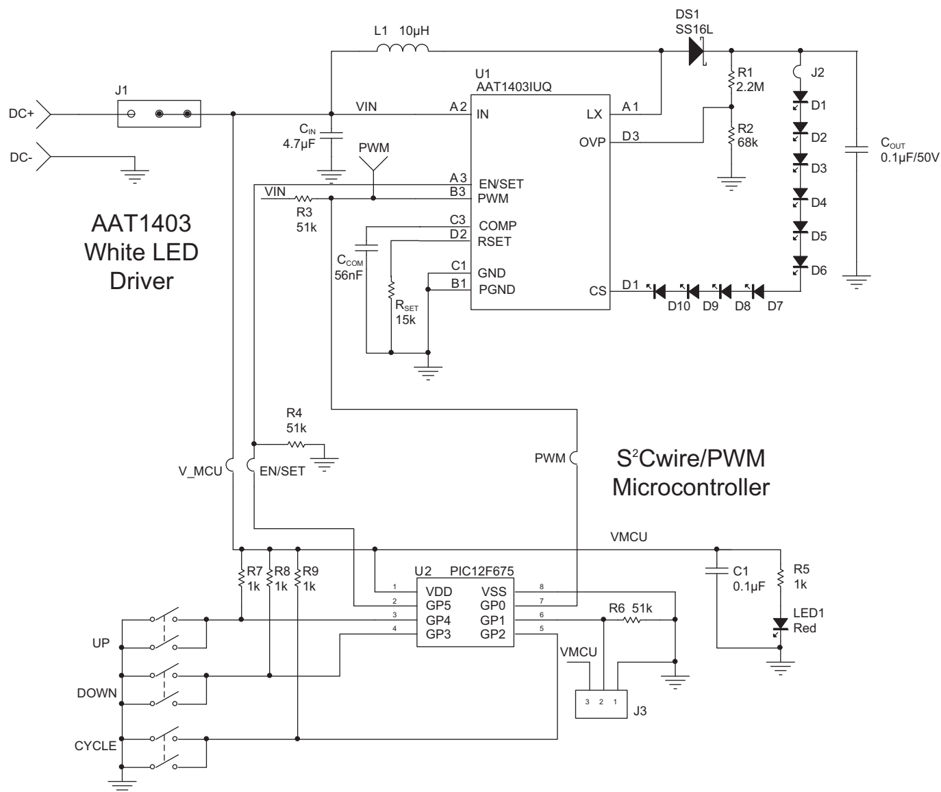
Figure 5: AAT1403 Evaluation Board Schematic.
