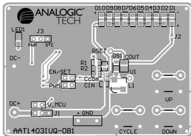
Figure 6: AAT1403 Evaluation Board Top Side Layout.
