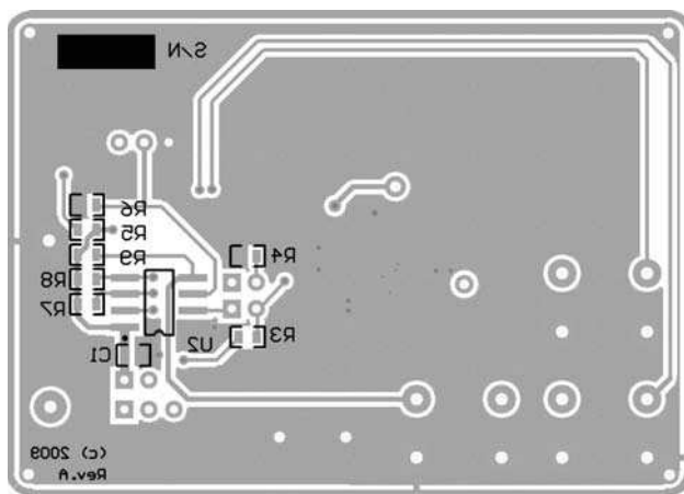
Figure 8: AAT1403 Evaluation Board Bottom Side Layout.
