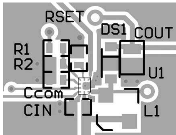
Figure 7: AAT1403 Evaluation Board Top Side Layout (detail).
