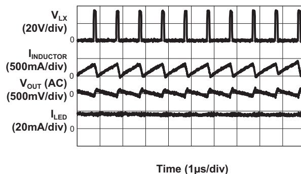
Operation Waveform
