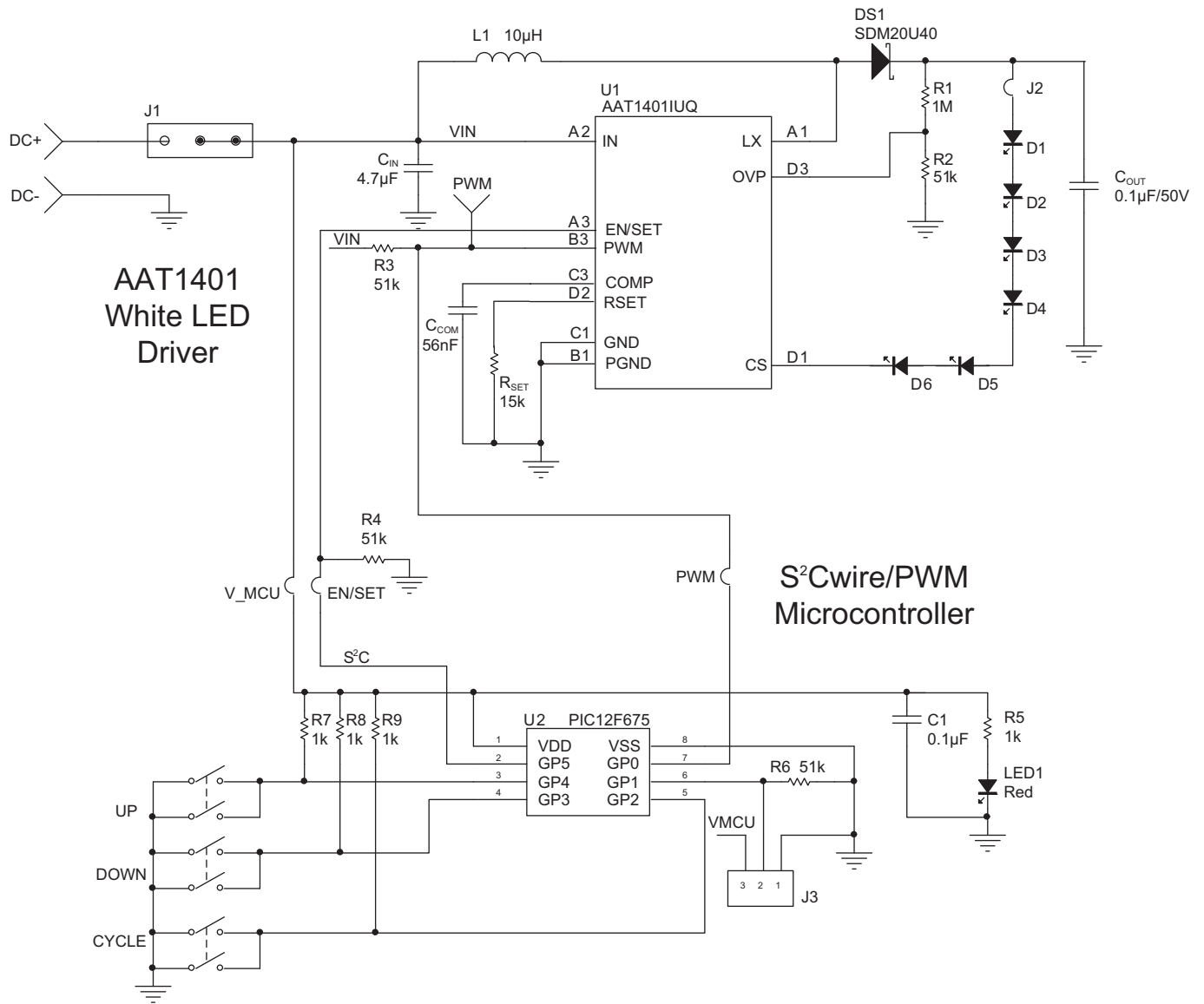
Figure 6: AAT1401 Evaluation Board Schematic.
