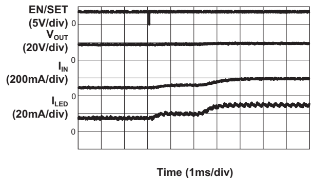
LED Current Transient by S 2 Cwire
