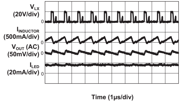
Operation Waveform
