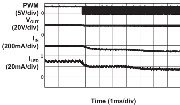
LED Current Transient
