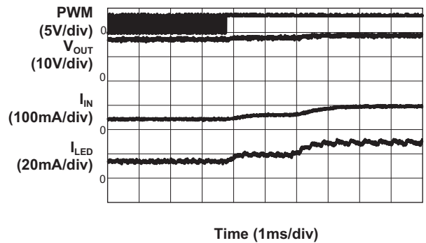
LED Current Transition
