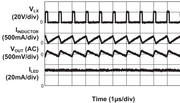
Operation Waveform
