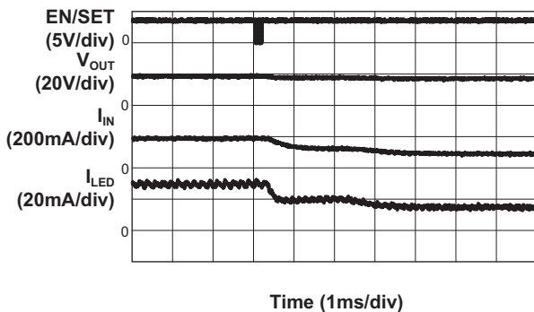
LED Current Transient by S 2 Cwire
