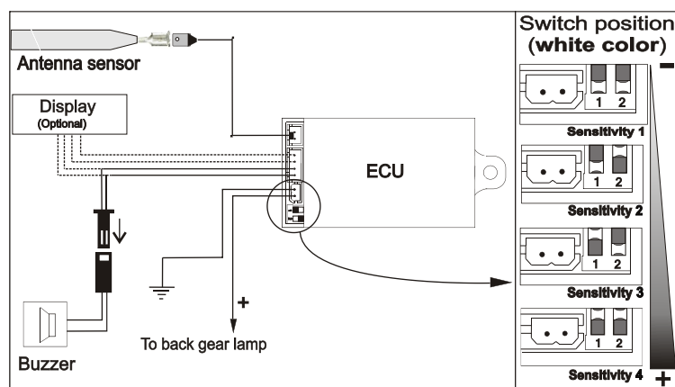
Block Schematic
