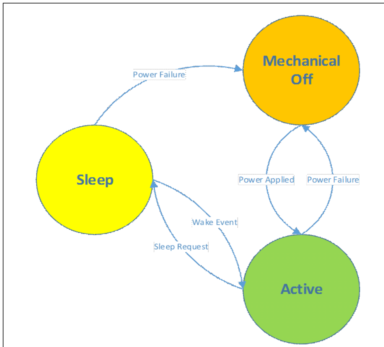
Figure 4-1. Power state change diagram
