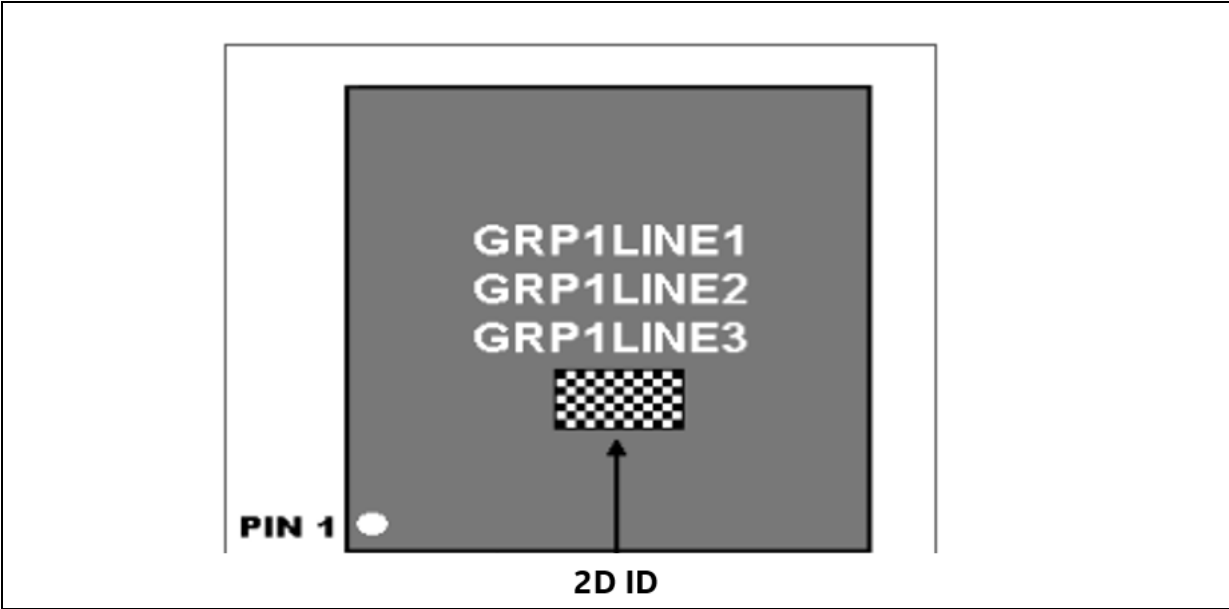
Figure 5-1. Package marking
